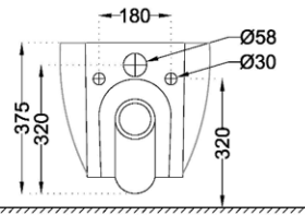
BACK VIEW
