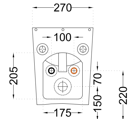
BACK VIEW A
